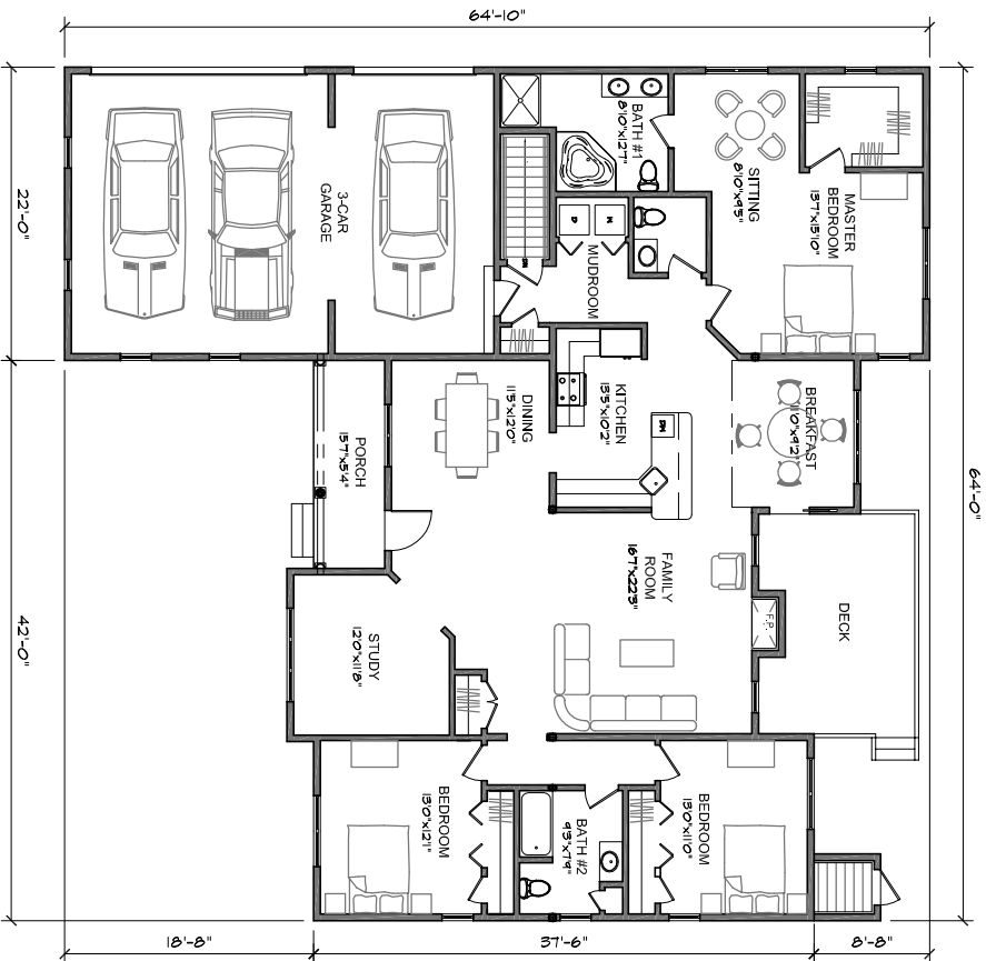
FLOOR PLAN
