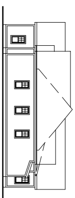
SIDE ELEVATION
