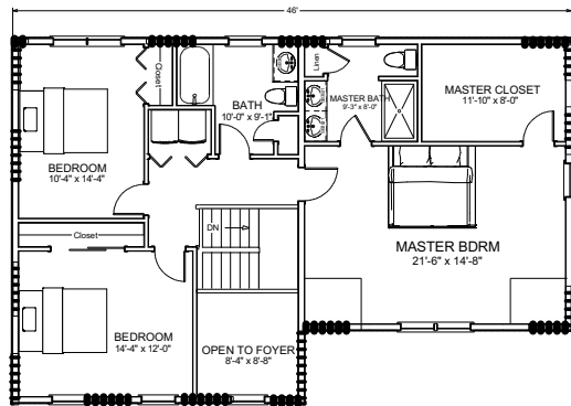
2nd Floor
